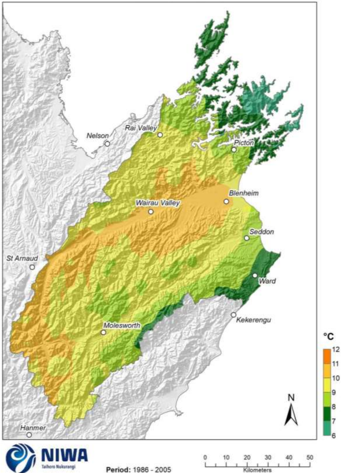
Figure 4-22: Modelled annual diurnal temperature range (Tmax minus Tmin), average over 1986-2005. Results are based on dynamical downscaled projections using NIWA's Regional Climate Model. Resolution of projection is 5km x 5km
