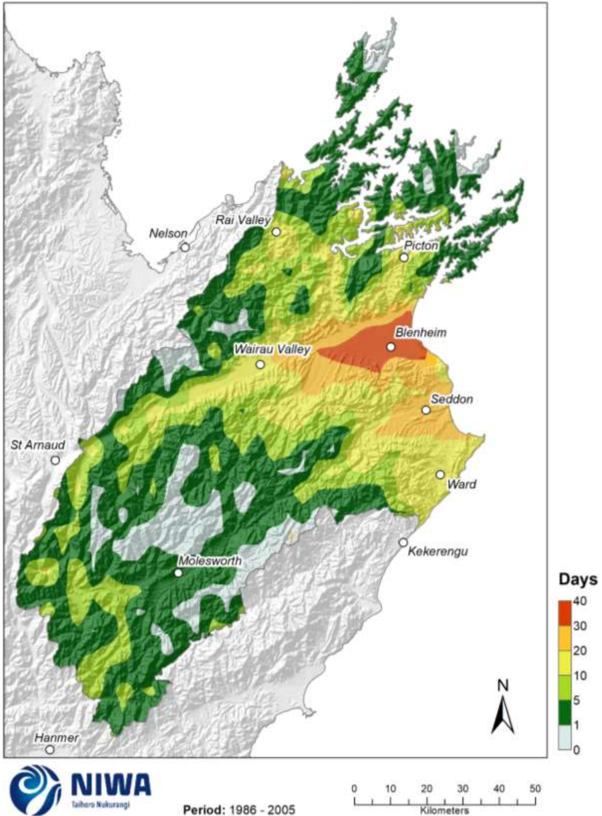
Figure 4-29: Modelled annual number of hot days (days with maximum temperature \geq 25^{\circ}\text{C} ), average over 1986-2005. Results are based on dynamical downscaled projections using NIWA's Regional Climate Model. Resolution of projection is 5km x 5km.
