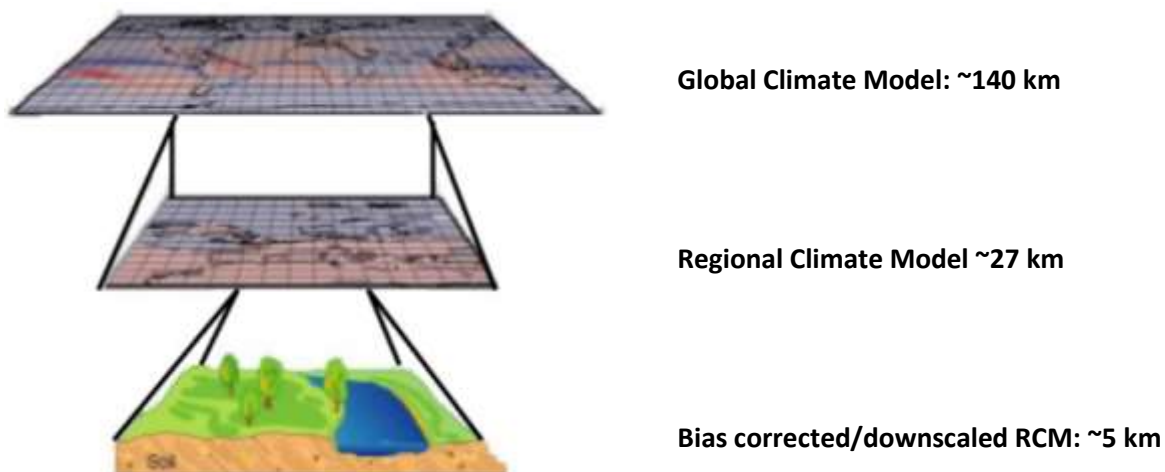
Figure 2-1: Schematic diagram showing the dynamical downscaling approach.
