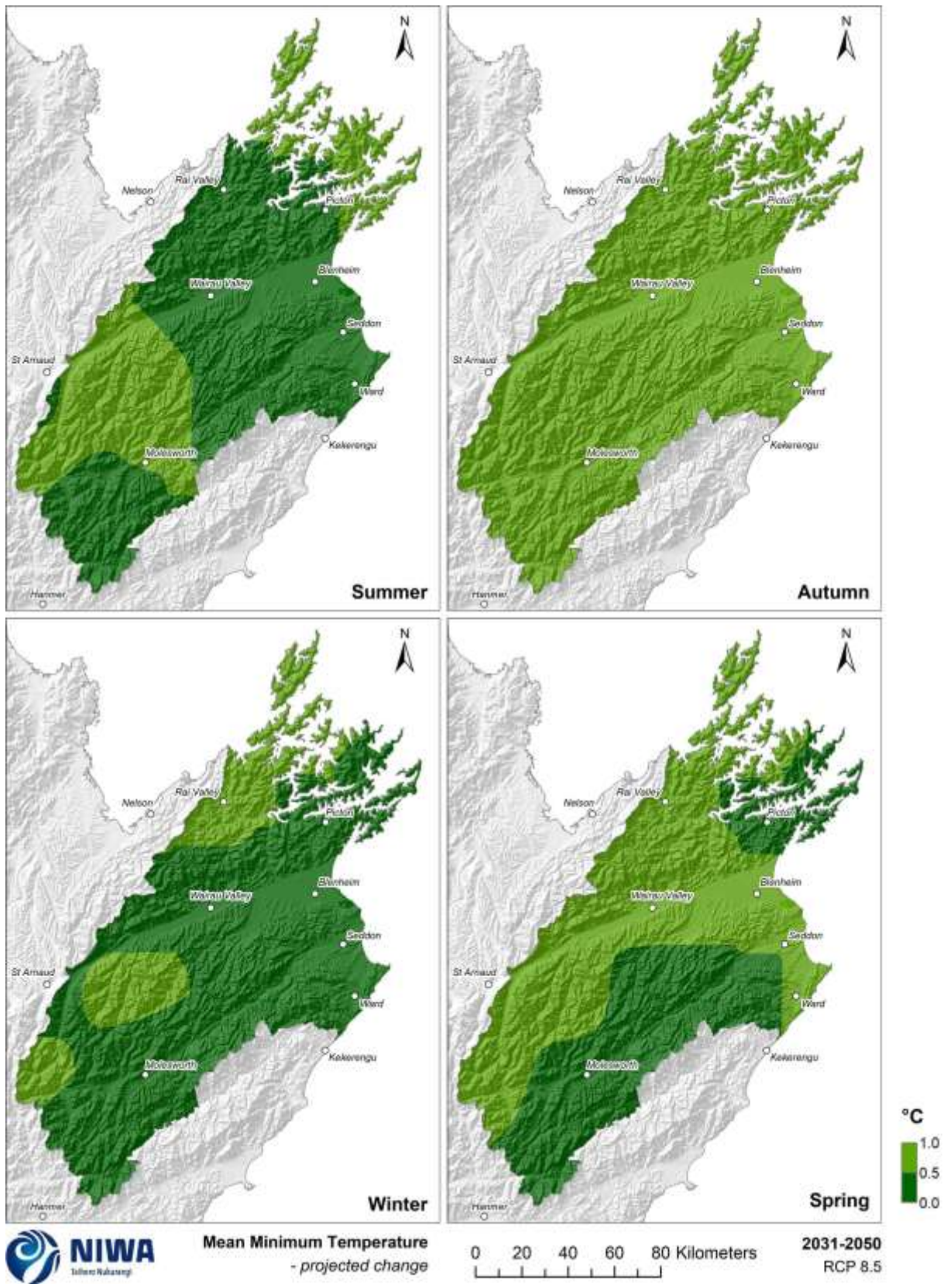
Figure 4-20: Projected seasonal mean minimum temperature changes by 2040 under RCP8.5. Relative to 1986-2005 average, based on the average of six global climate models. Results are based on dynamical downscaled projections using NIWA's Regional Climate Model. Resolution of projection is 5km x 5km.
