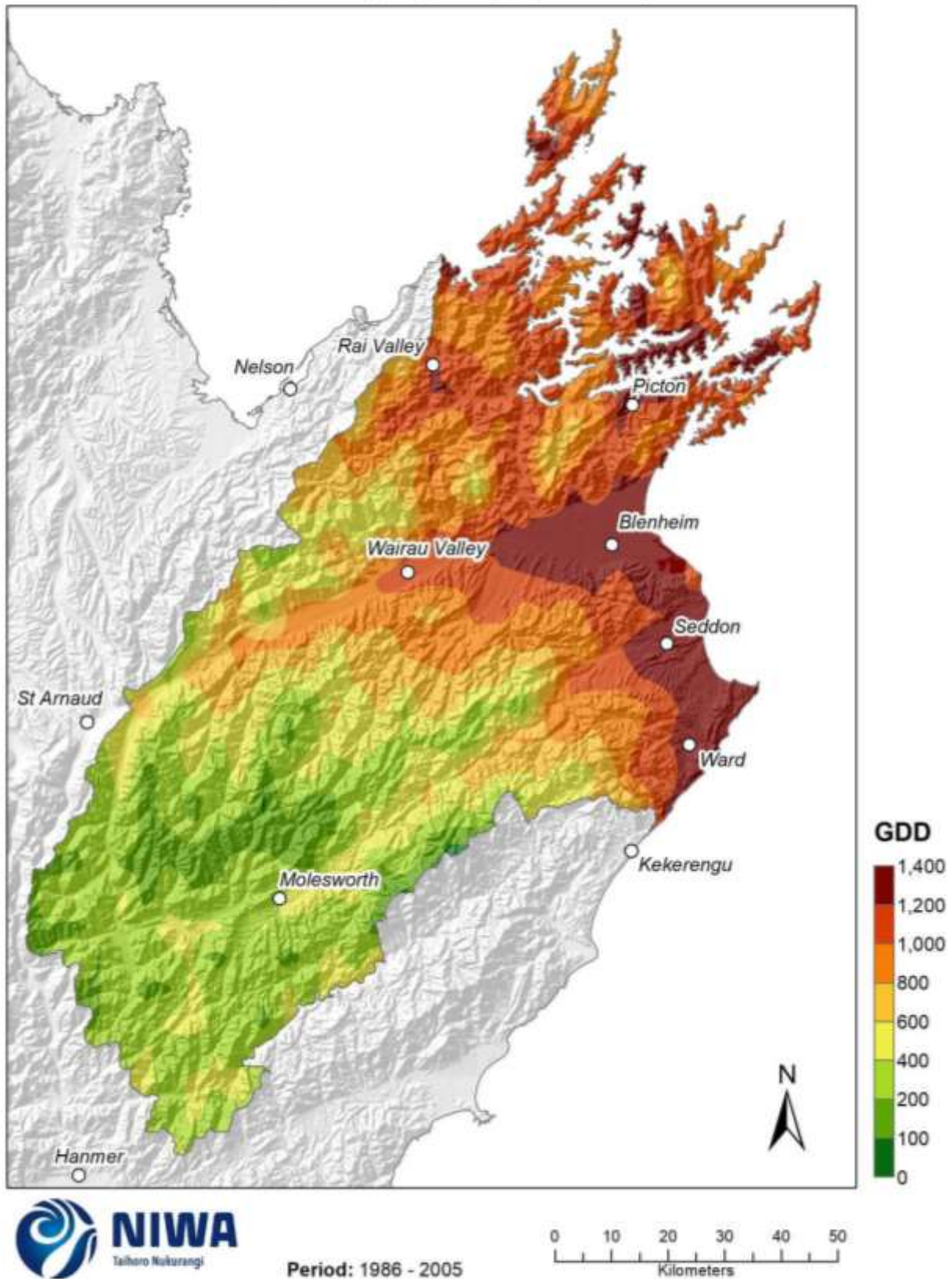
Figure 4-31: Median annual Growing Degree-Days (GDD) base 10°C. Results are based on dynamical downscaled projections using NIWA's Regional Climate Model. Resolution of projection is 5km x 5km.
