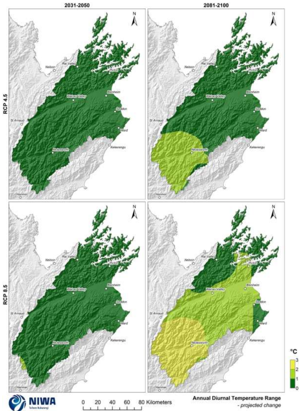
Figure 4-23: Projected annual diurnal temperature range (Tmax minus Tmin) changes at 2040 (2031-2050 average) and 2090 (2081-2100 average) for RCP4.5 and RCP8.5. Relative to 1986-2005 average, based on the average of six global climate models. Results are based on dynamical downscaled projections. Resolution of projection is 5km x 5km.
