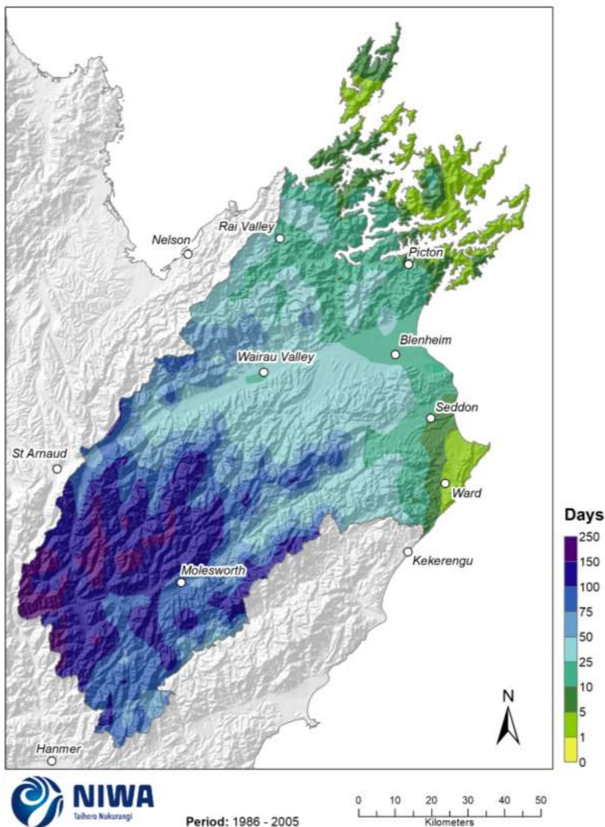
Figure 4-24: Modelled annual number of frost days (daily minimum temperature \leq 0^{\circ}\text{C} ), average over 1986-2005. Results are based on dynamical downscaled projections using NIWA's Regional Climate Model. Resolution of projection is 5km x 5km
