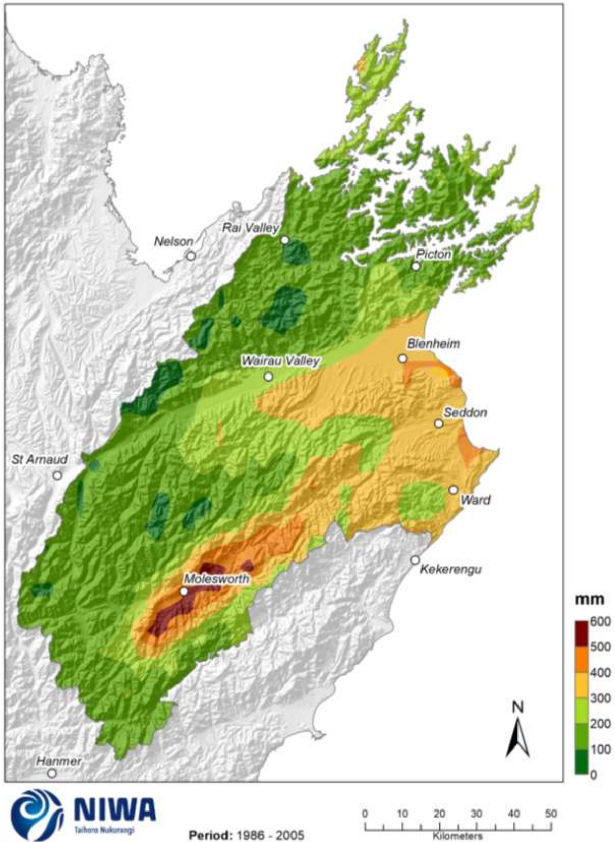
Figure 6-1: Modelled annual potential evapotranspiration deficit accumulation (mm), average over 1986-2005. Results are based on dynamical downscaled projections using NIWA's Regional Climate Model. Resolution of projection is 5km x 5km.
