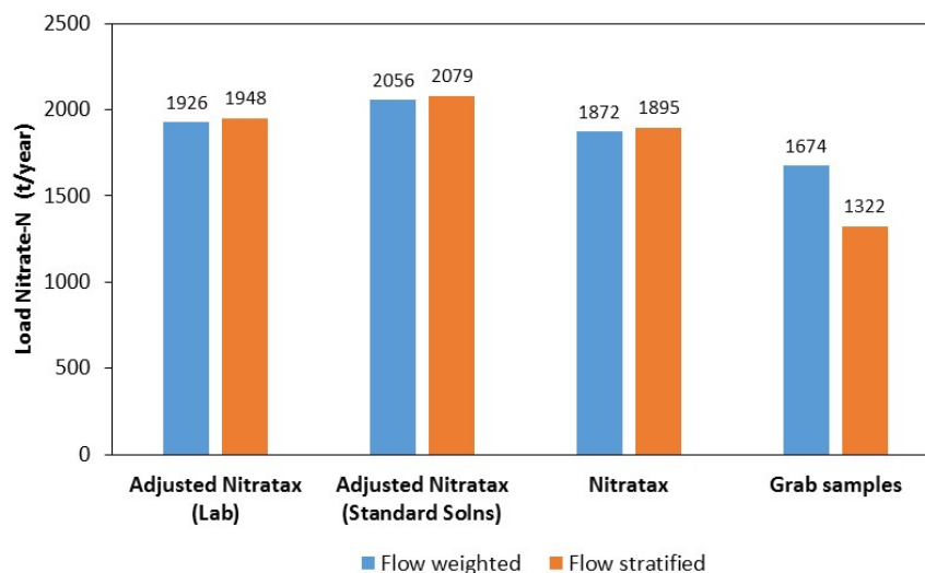
Fig. 7. Comparison of the annual nitrate-N loads calculated using the adjusted and non-adjusted high-resolution NITRATAX sensor and the monthly grab sample method in the Manawatu River at the Teachers College monitoring site, from Feb 2016 to Jan 2017. The nitrate-N loads (t/year) were calculated using the flow-weighted and flow-stratified river load calculation methods, with actual loads denoted above the bars.
