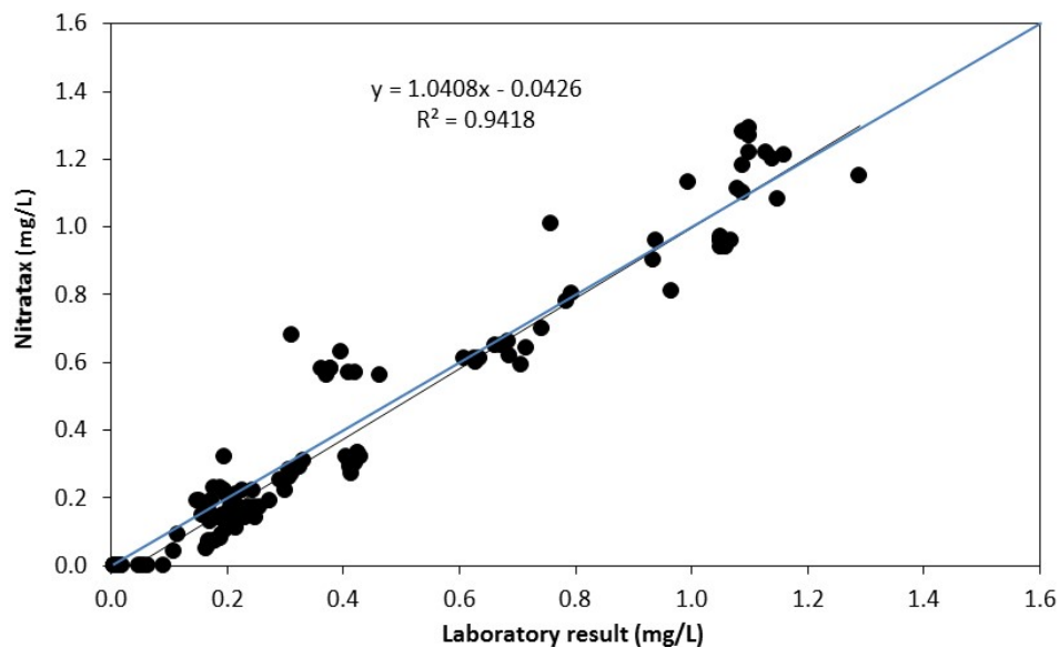
Figure 1. Calibration between laboratory measured and NITRATAX nitrate-N concentrations [adjusted NITRATAX value = (\text{NITRATAX} + 0.0426)/1.0408 ]. The blue line is the 1:1 line.
