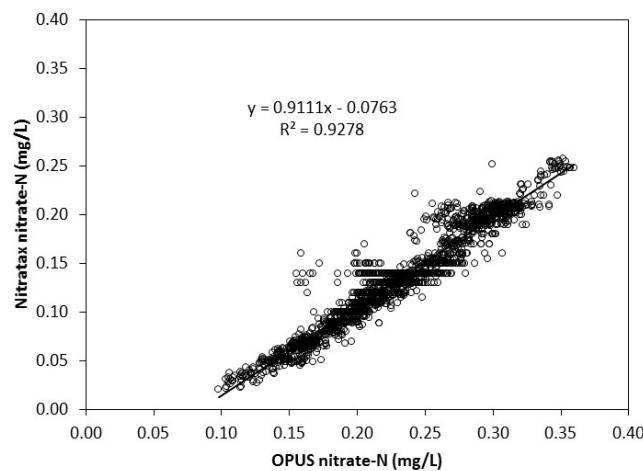
Figure 10. Comparison of the unadjusted nitrate-N concentrations measured by the OPUS and NITRATAX sensors from 20 Dec 2016 to 2 Jan 2017 and 16 Jan to 23 Jan 2017 in the Manawatu River at the Teachers College monitoring site.
