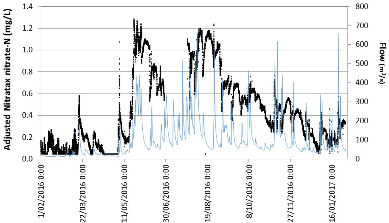
Figure 5. Changes in adjusted NITRATAx nitrate-N concentrations (black circles) in relation to river flow rate (blue line), from Feb 2016 to Jan 2017, in the Manawatu River at the Teachers College monitoring site.
