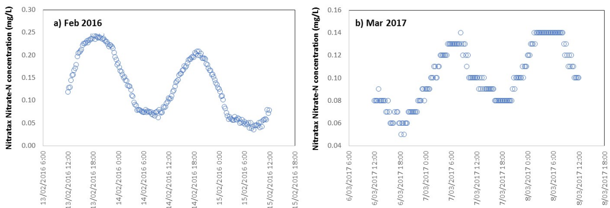
Figure 4. Comparison of diurnal variations in unadjusted NITRATAX nitrate-N concentrations measured in (a) Feb 2016 and (b) Mar 2017, in the Manawatu River at the Teachers College monitoring site.
