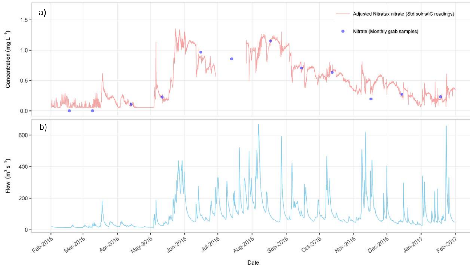
Figure 8. Comparison of nitrate-N concentrations measured by a) monthly grab samples (blue circles) and adjusted NITRATAx concentrations (red line) and b) flow rate (m 3 /s) (blue line), from Feb 2016 to Jan 2017, in the Manawatu River at the Teachers College monitoring site.
