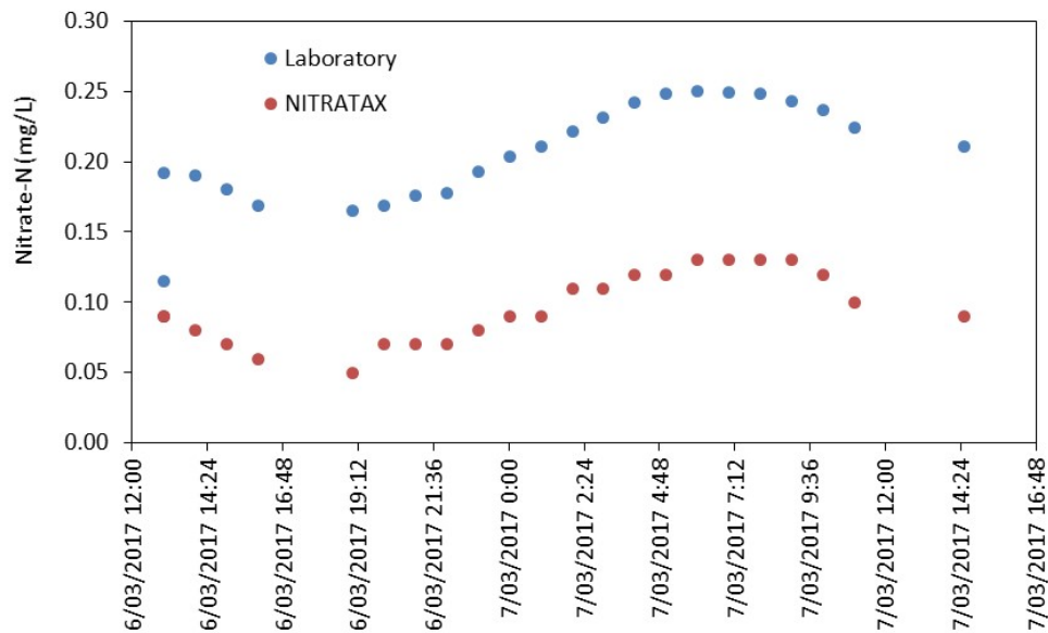
Figure 3. Comparison between the unadjusted NITRATAX nitrate-N concentration and nitrate-N concentrations measured using the laboratory grab sampling method over a ~24 hr period on March 6-7 2017, in the Manawatu River at the Teachers College monitoring site.
