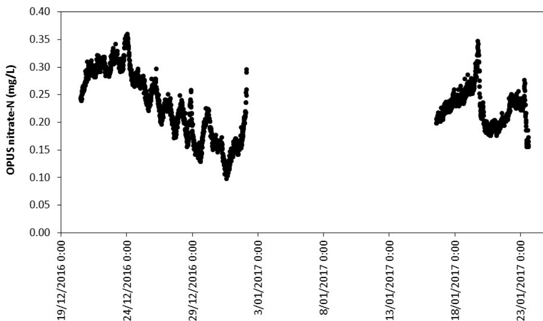
Figure 9. Nitrate-N concentrations measured by the OPUS sensor for two periods of measurement (20 Dec 2016 to 2 Jan 2017 and 16 Jan to 23 Jan 2017) in the Manawatu River at the Teachers College monitoring site.
