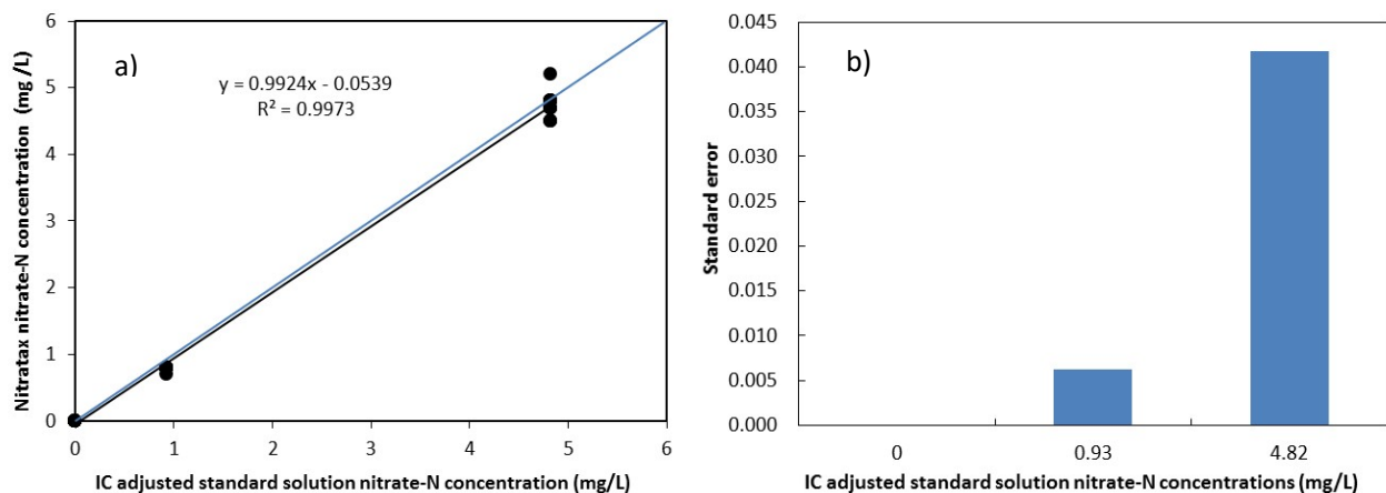
Figure 2. a) Calibration between ion chromatography measured standard solutions and NITRATAX nitrate-N concentrations [adjusted NITRATAX value = (NITRATAX + 0.0539)/0.9924] and b) standard error around the mean for NITRATAX nitrate-N concentrations when calibrated against ion chromatography measured standard solutions. The blue line is the 1:1 line.
