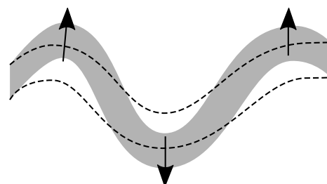
Figure 2-26 Mechanisms of meander belt evolution on the Waiapu.
