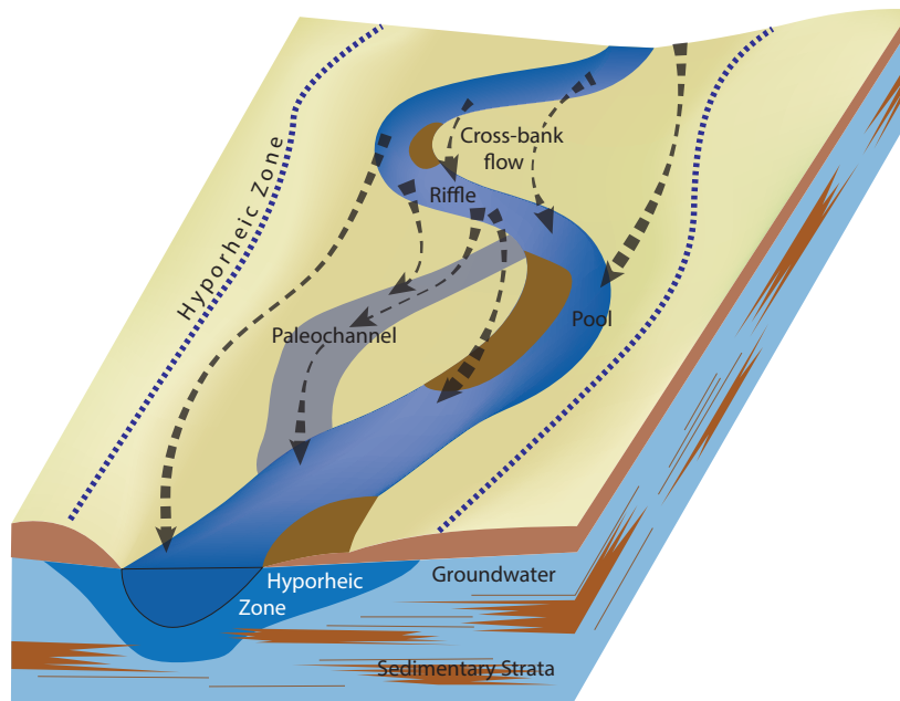
Figure 2-7 Water pathways through the hyporheic zone in gravel bed rivers provide linkages for oxygen and nutrient flux, which are important for stream biota forming the basis of the riverine food web. Preferential flow may occur in abandoned paleochannels. Alteration of these pathways can impact the potential for ecological recovery of the river. After Tonina and Buffington (2009).
