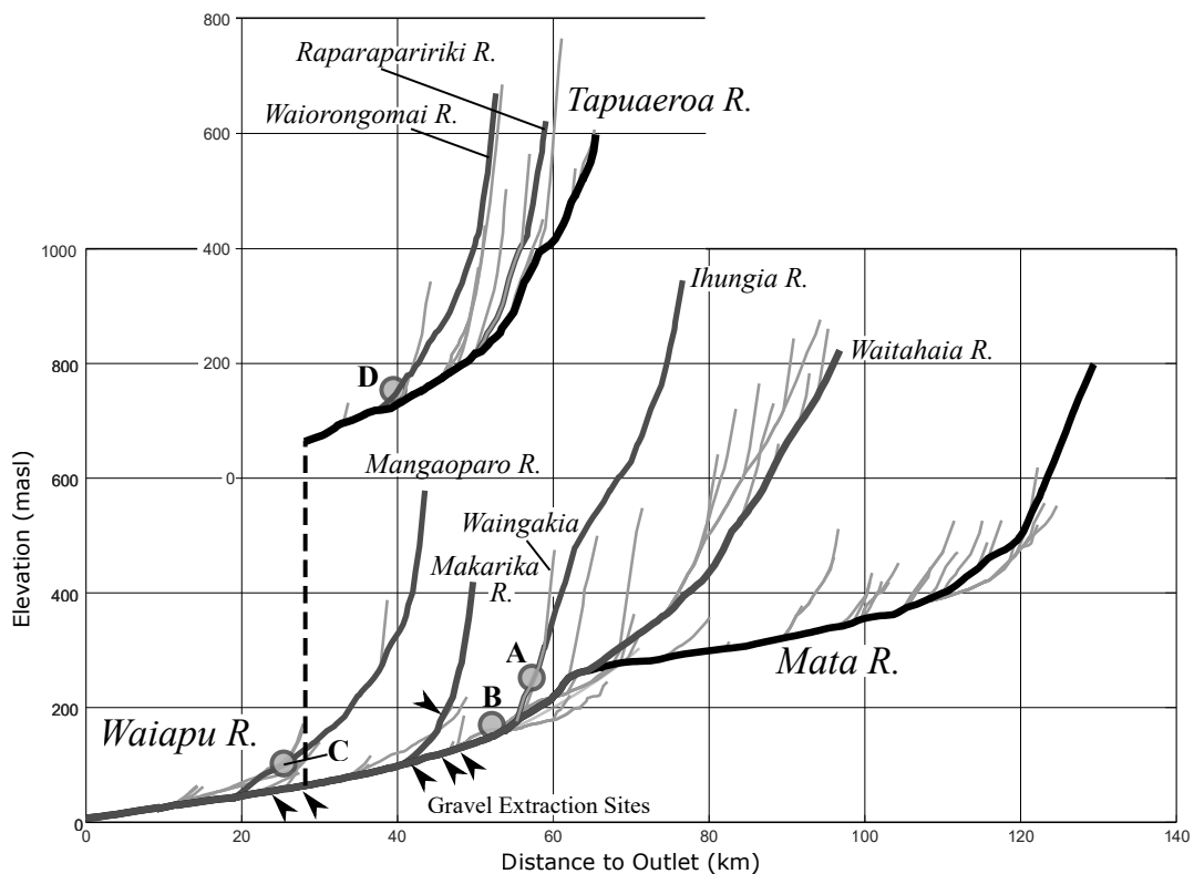
Figure 2-17 Longitudinal profile of Waiapu River and its tributaries. Letters with circle symbol indicate location of sample reaches discussed in the text, and pictured in subsequent figures.
