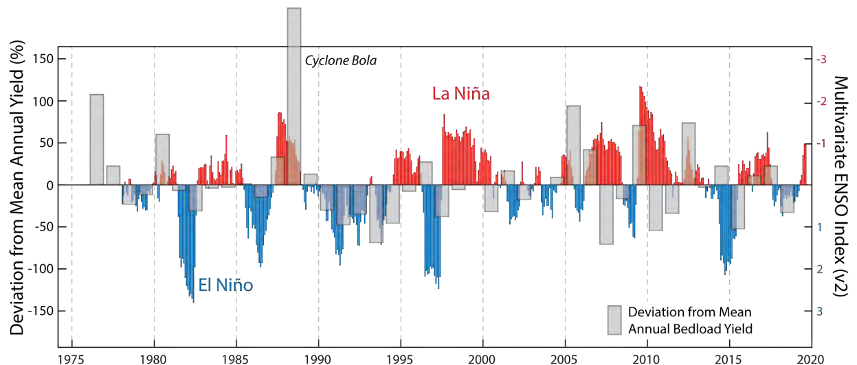
Figure 3-40 Cross-section-based modelling of bedload transport, based on the annual flow duration curves for flows from 1976 to 2019. We used the Wilcock-Crowe (2003) equation, basing calculations on sediments and hydraulic conditions within the study site near Rotokautuku Bridge. The bar chart shows yield as a percentage deviation from the long term mean ('0'). Wet years may have twice as much bedload (+100%) relative to the long term mean; dry years will have less (-80%). The Multivariate El Niño/Southern Oscillation (ENSO) Index refers to the variation in sea surface temperatures across the equatorial Pacific Ocean and surface atmospheric pressure in the tropical Pacific (cf. Mullan, 1995; Mosley, 2000). This trend can strongly influence New Zealand storm climate, and the setup of weather systems. While it is not a perfect relationship, it does provide some insight into the longer-term controls on gravel yield, and the significant decadal-scale variability.
