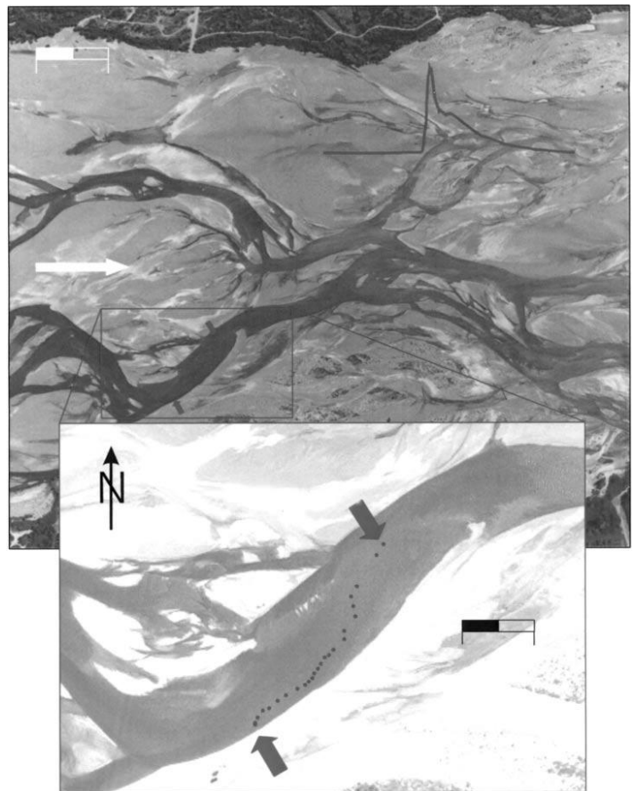
Figure 3-31 Habersack (2000) used radio-tagged particles to trace the transport path of grains on the bed of the Waimakariri River at Crossbank. The lower figure shows the resting positions of the grain as it moves from erosion site to deposition site on the rising and falling limb of a flood hydrograph.
