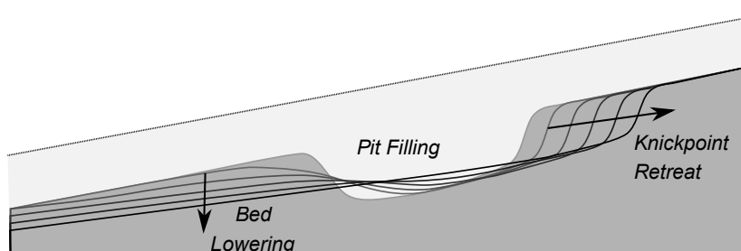
Figure 2-11 Conceptual diagram showing the effects of deep pit excavation within a riverbed (diagram adapted from Kondolf (1994)). The scale and proportions of these erosional effects will vary, depending on river scale, sediment supply, and other hydraulic and sedimentary factors.
