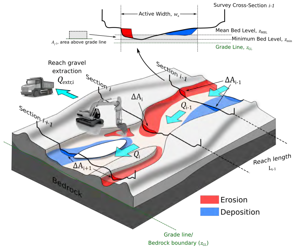
Figure 3-32 A schematic showing typical gains and losses within a reach. Note that reaches are set to roughly the transport path length. The gains and losses are weighed up for each reach ( \dots i-1, i, i+1 \dots ), and the balance is routed downstream as sediment discharge ( Q ). If the downstream cumulative balance remains close to zero (gains and losses cancel out), then the system is considered to be in equilibrium. If there are more gains than losses along the reaches, the system aggrades, building up the bed; and vice-versa, with systematic losses, the system degrades.
