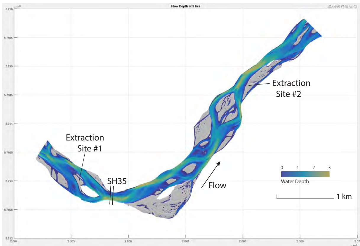
Figure 3-37 Delft3D model of the Waiapu River with discharge at 600 \text{ m}^3\text{s}^{-1}
