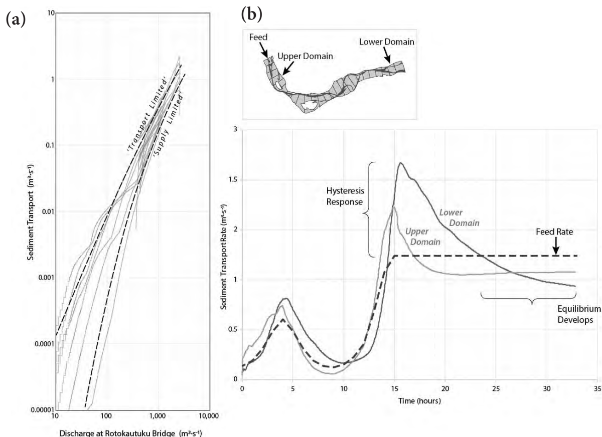
Figure 3-38 Transport rates observed in 1D and 2D, live-bed Delft3D morphodynamic model. (a) Transport rating relationships, based on 1D and 2D simulations of bedload transport along the study reach. (b) Time series from a model run, showing the highest feed rate that could be maintained without substantial riverbed aggradation. The river hydrograph was ramped up to 3000 m^3 \cdot s^{-1} with a maximum feed rate of 1.5 m^3 \cdot s^{-1} (making the assumption 1 m^3 = 1600 kg ) The results show that in the early stage of model 'spin-up' the river can deliver material above the feed rate, as material is eroded from within the reach. Eventually, the model establishes an equilibrium and rates adjust to more effectively transfer the rate fed from upstream. We refer to these initial conditions as being 'transport limited', where the river has an effectively unlimited supply of bedload from upstream, and 'supply limited', where within-reach supply has been exhausted, and the upstream supply becomes limited by the variable conveyance capacity along the river, and delivery of material falls more or less into line with the supplied rate from upstream.
