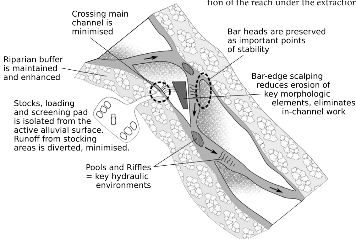
Figure 4-44 Site design to minimise impacts on ecological and geomorphic processes within the extraction reach. Operations should stay out of flowing water where possible, minimise impact on channel morphology and prevailing grain size distribution in the river, and maintain and protect the riparian zone between the channel and surrounding environment.
