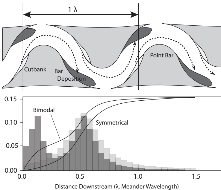
Figure 3-30 The transport path length of a given bedload particle is thought to extend about one half of a meander wavelength: from erosion at a scour zone or outside bend, to deposition downstream of the next point bar, for instance. In laboratory experiments, Pyrcie and Ashmore (2003) observed cases where most deposition occurred either close to source (leading to a bimodal distribution), or around 0.5 \lambda , near the next point bar downstream (symmetrical). Thus, the dominant wavelength should provide a good first-order estimate of \langle L \rangle for long-term average transport rate estimates.
