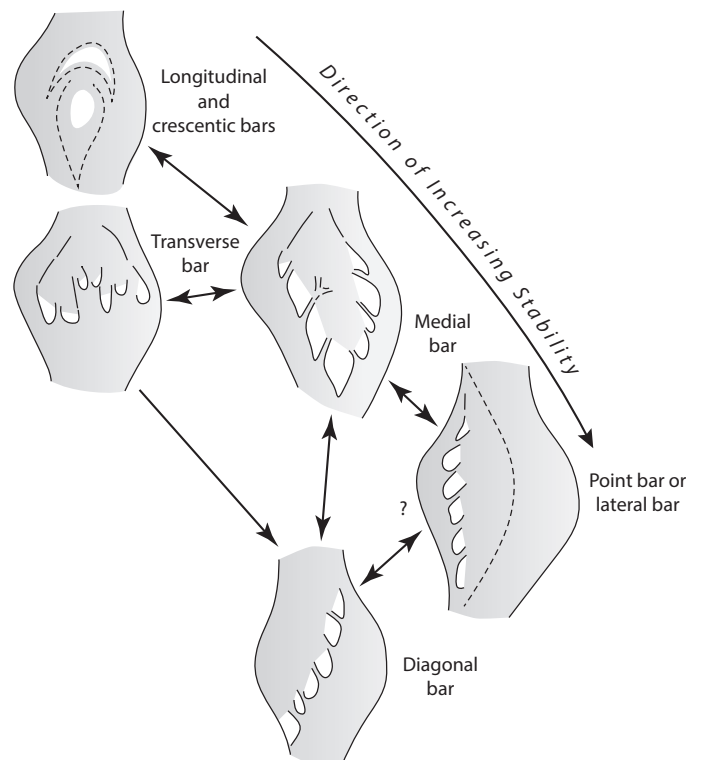
Figure 2-24 The relative stability of bar types within braided to wandering gravel bed rivers, according to Kellerhals et al. (1976). The Waiapu tends to exhibit the more stable medial, lateral and diagonal bars, indicative of relatively high rates of sediment transport, though perhaps not as high as a more intensively braided system.
