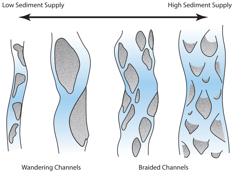
Figure 2-16 The influence of sediment supply on river morphology. System complexity and habitat diversity increase with higher rates of sediment transfer, though optimum ecological conditions are thought to be in the mid- to high range of this spectrum (see Piegay et al., 2006 for further details).
