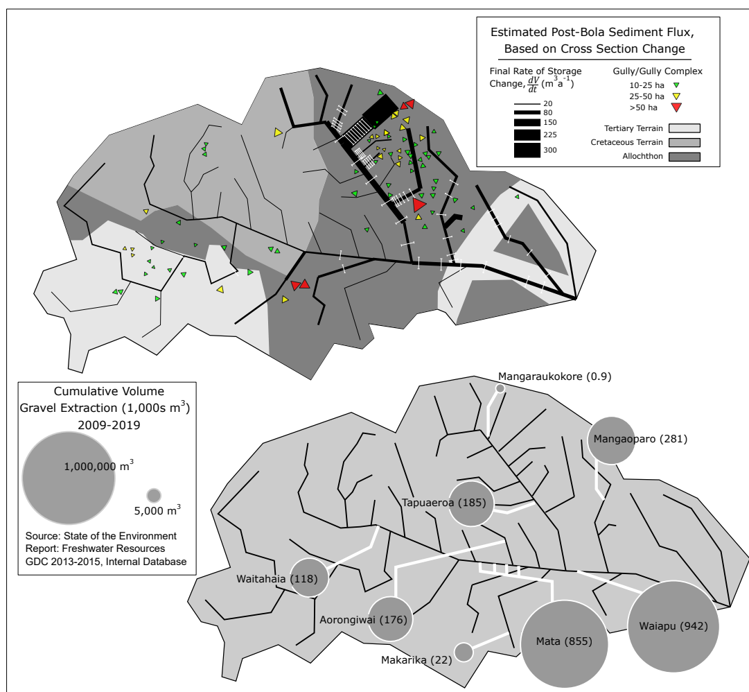
Figure 2-14 (Top) Schematic of the catchment, showing the river network and cross-section monitoring sites. The thickness of the lines reflects the relative rates of sediment flux, based on changes observed in cross-section measurements since 1988 (see Tunnicliffe et al. , 2018). (Bottom) Sites of gravel extraction within the Waiapu catchment active and reporting between 2009 and 2019. Volumes were consented, but not necessarily extracted.
