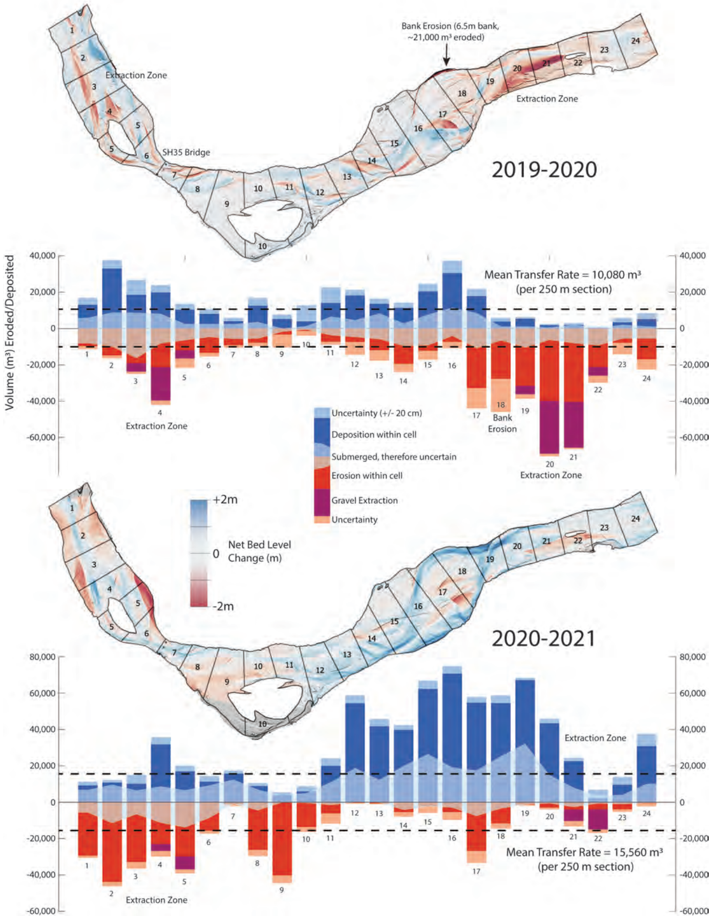
Figure 3-35 Digital Elevation Model (DEM) of Difference, for the Waiapu River, extending 6 km from the Tapuaeroa-Mata confluence to (roughly) Walker Road. Shading on the map shows the magnitude of erosion (red) and deposition (blue) from three successive surveys between April 2019 and February 2021. See text for further details.
