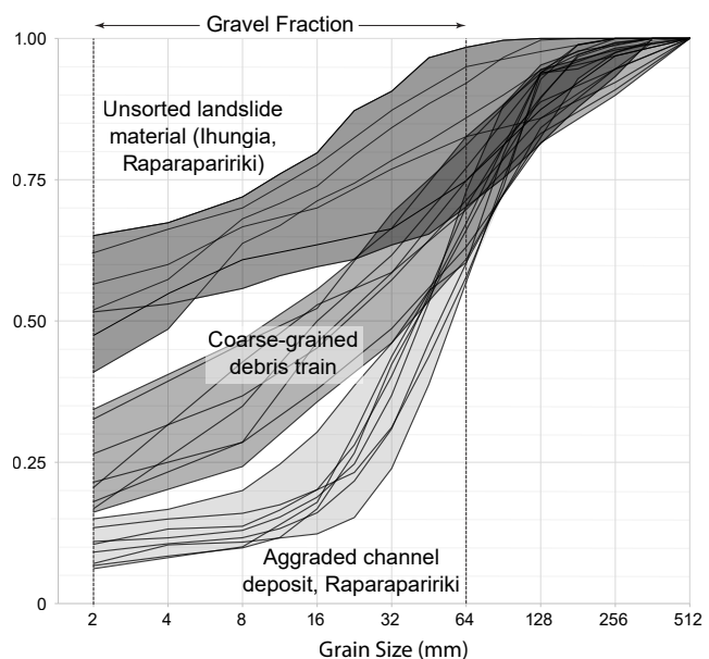
Figure 2-15 Surface grain size characteristics, sample by point counts of surface gravels. The subsurface material (not shown here) tends to be more enriched in sand and silt fractions.
