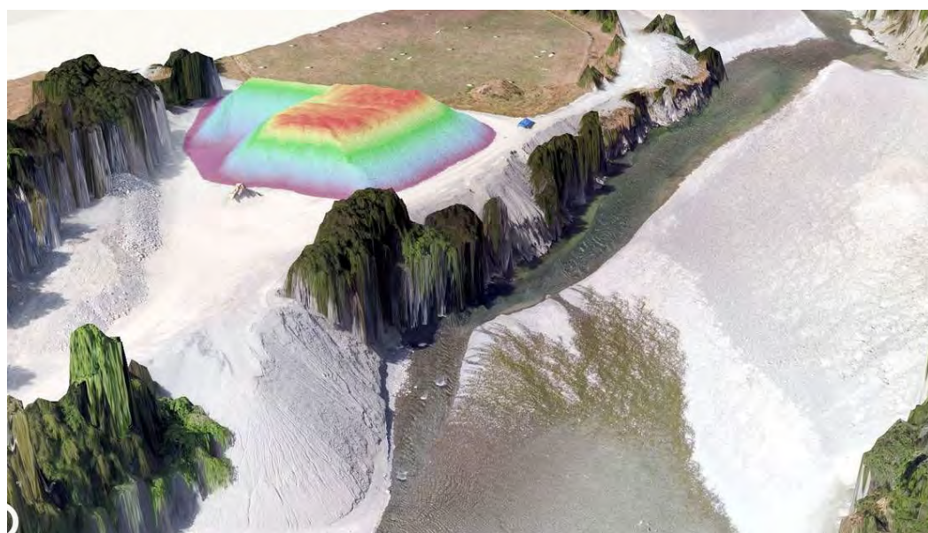
Figure 3-41 Oblique view of a digital SfM model (2cm resolution). A stockpile of gravel taken from the Mata River, off of Horehore Road is highlighted, with colours representing the relative height of the pile (up to 10 m). With Structure-from-Motion and point cloud processing software, discrete volumes of cut and fill quantities can be quickly assessed with relative precision on the order of 1-2%.
