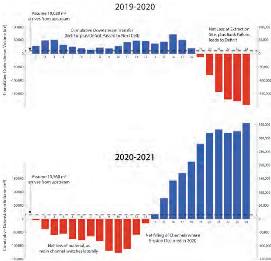
Figure 3-36 Longitudinal charts showing cumulative downstream sediment transfer, based on the gains and losses within each cell of the survey (charts in Figure 3-35). The balance of cut and fill in a cell is routed to the next cell downstream: a series of cells with net losses will lead to progressive lowering of the trend into the red (negative values); likewise serial gains will lead to a rise in the trend. Perfectly balanced gains and losses in series will produce a horizontal line.
