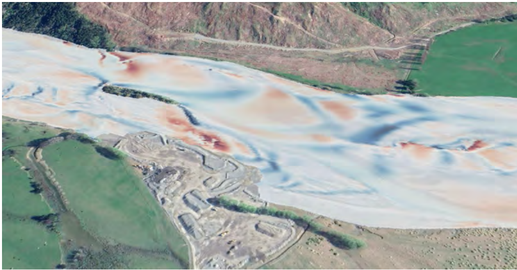
Figure 3-39 Waiapu River near the Walker Road extraction site. Bedload transport within the Delft3D model consists of migrating lobes of gravel moving along the river bed, shaping (and being shaped by) river flows. The transit of these bedforms is another reason for the highly non-linear transport rates observed in the model, and the lagged response to changing sediment feed rate at different cross-sections over time. Red denotes erosion (troughs) and blue is deposition (peaks) of the migrating bedforms.
