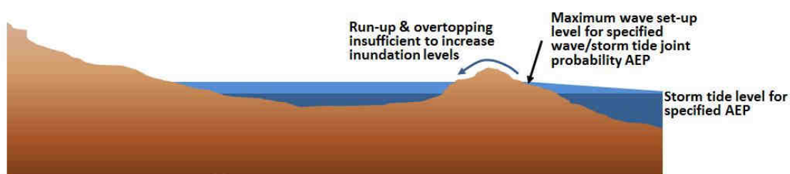
Figure 13 Storm tide / wave set-up levels and resulting inundation levels where wave run-up and overtopping do not increase inundation levels above those resulting from other inundation pathways (for example estuary or river mouth, or storm water connection).
