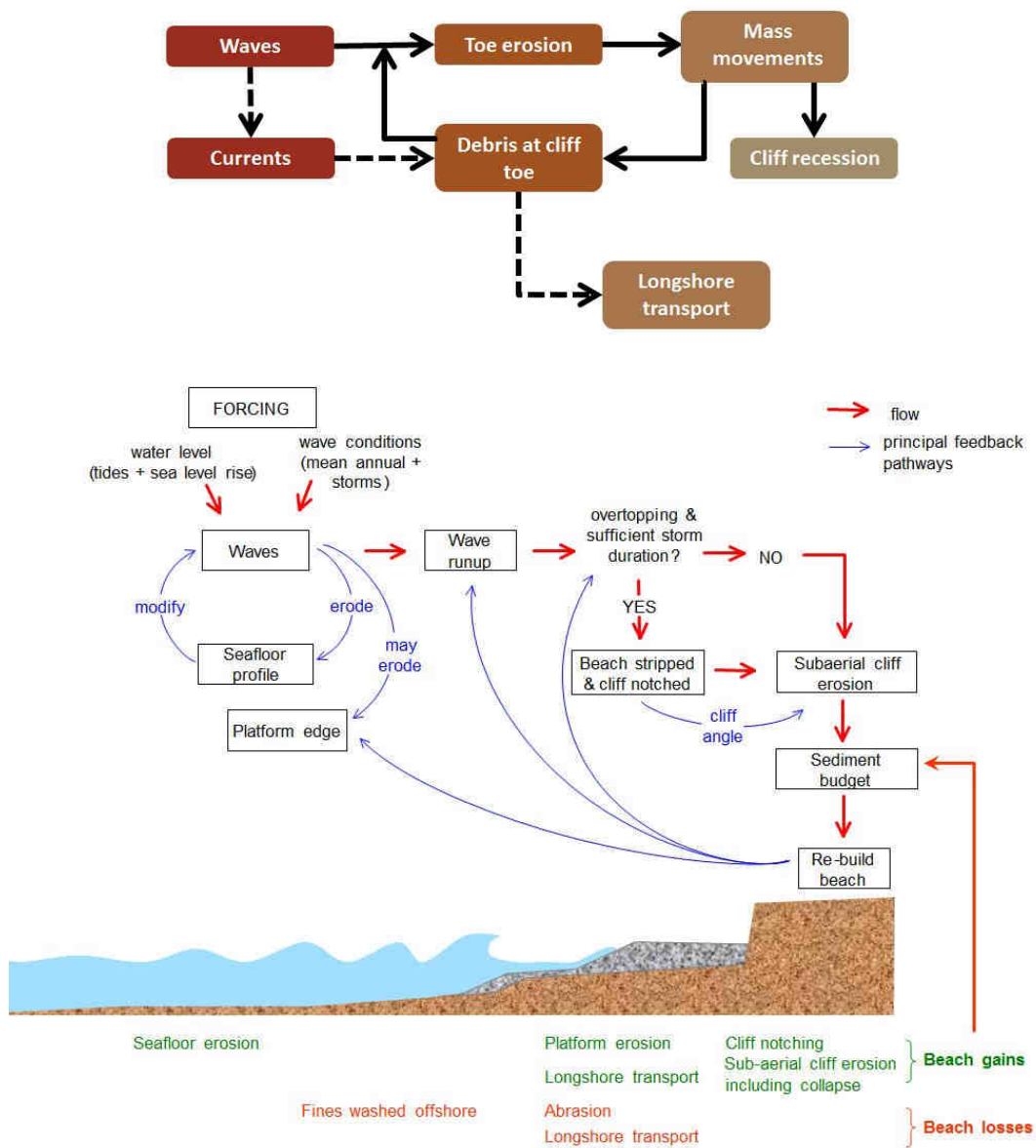
Figure 22 Examples of a simple (top) and more detailed (bottom) conceptual model of cliff erosion processes in South Canterbury (Courtesy Murray Hicks, NIWA).
