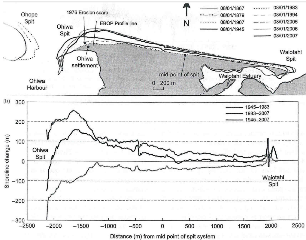
Figure 25 Shoreline position between Ohiwa and Waitoahi spits. Top: Geo-referenced historic shorelines. Bottom: analysis of shoreline change a 1 m intervals along the coastline. Adapted from Bryan et al, (2008).
