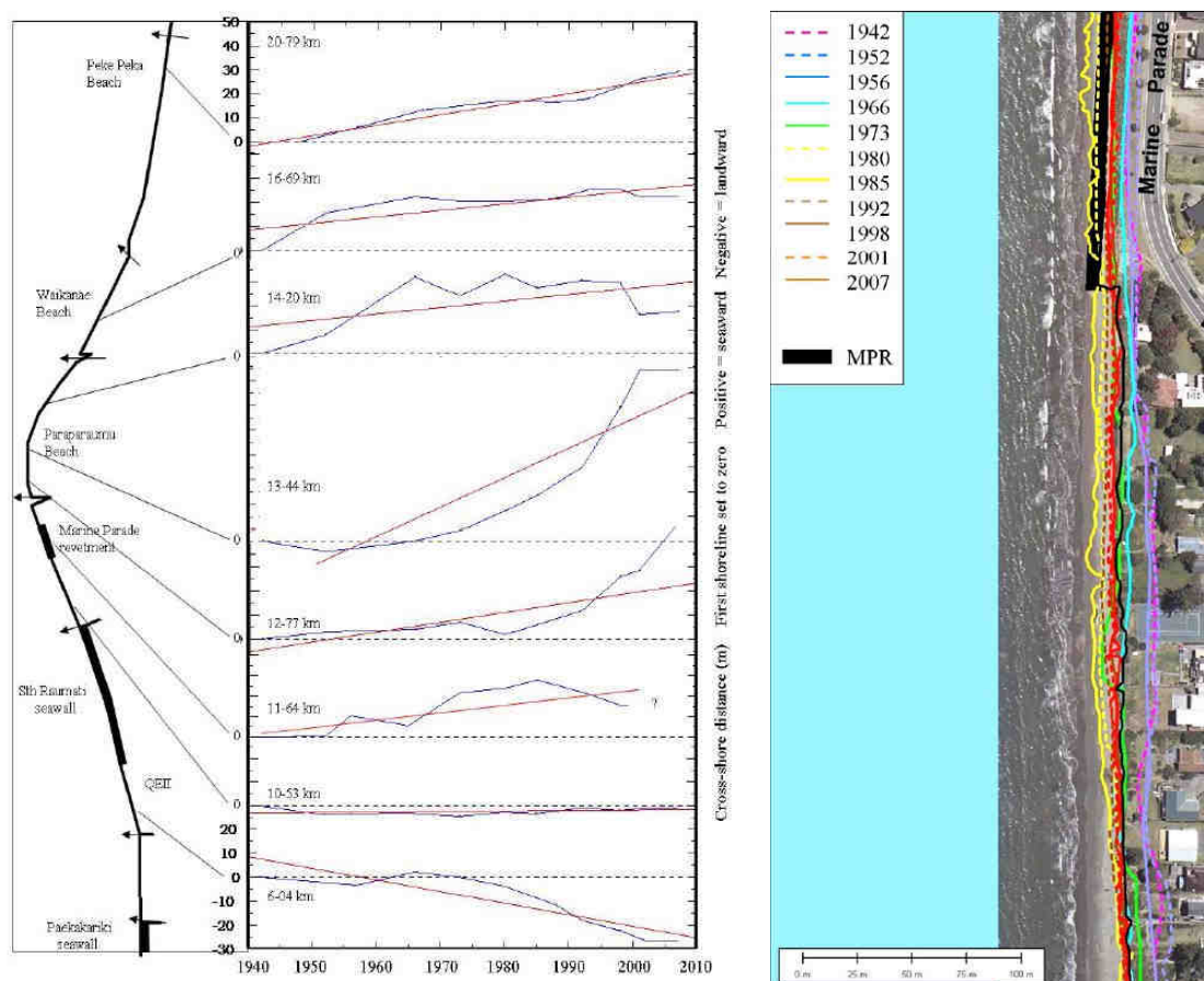
Figure 27 Example of linear shoreline change trends for various points (left), and shoreline position at various times between 1942 and 2007 for a section of the Kapiti coast. Source: Shand (2010).
