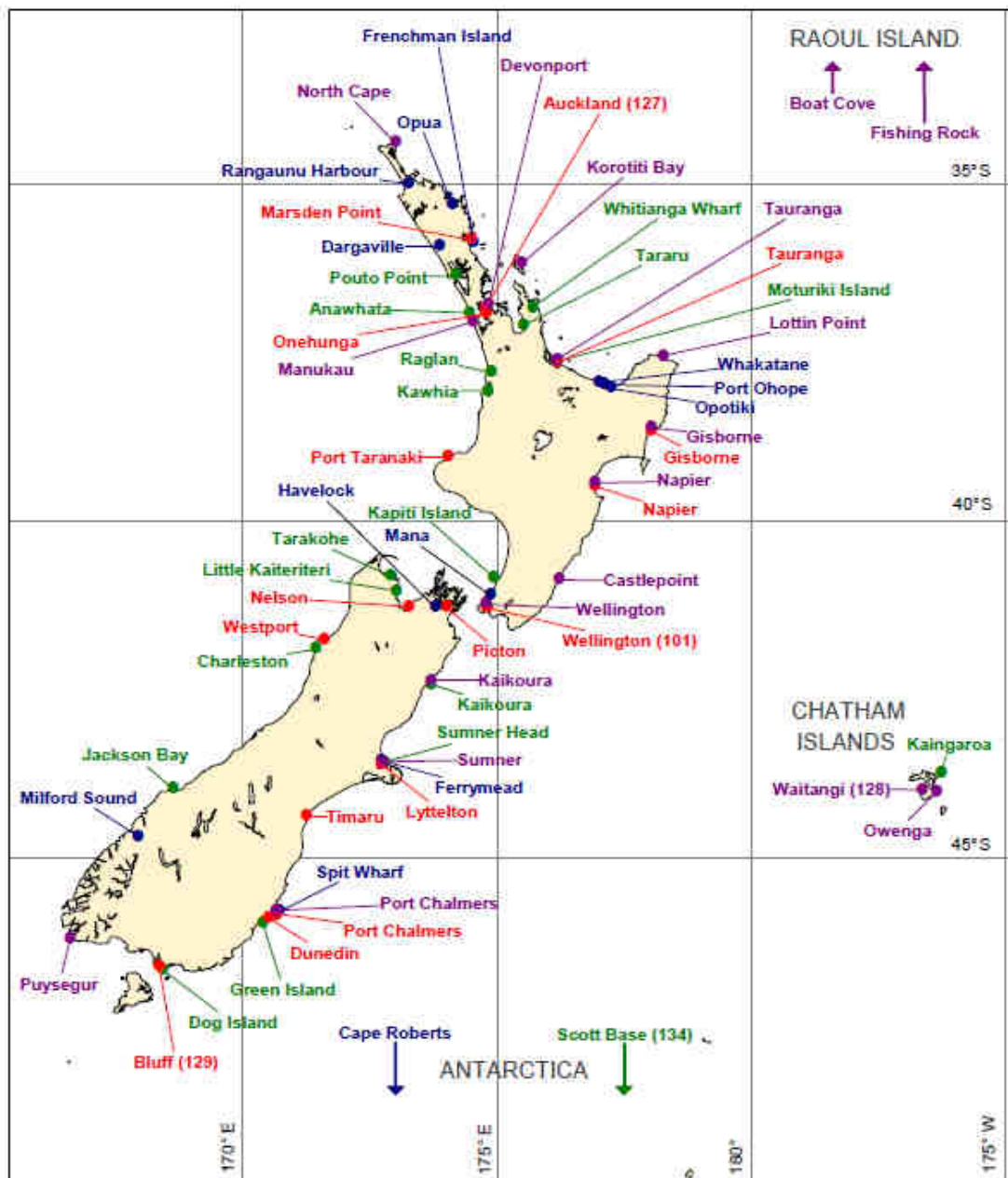
Figure 7 Locations of known sea level records which may be suitable for extreme storm tide analysis. The major port sites are shown in red, open coast sites shown in green, GeoNET tsunami monitoring sites shown in purple and other sites (except four Tauranga Harbour gauges) shown in blue. Source: Land Information NZ and NIWA
